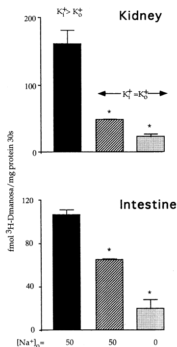
Fig. 3. 30 s sugar uptake into BBMVs in the presence and absence of electrical membrane potential and/or \text{Na}^+ chemical gradient. The BBMVs were loaded with a buffer consisting of (in mM): 140 mannitol, 50 KG and 50 HEPES-Tris (pH 7.5). The uptake buffer contained (in mM): 50 HEPES-Tris (pH 7.5), 0.045 valinomycin, 10^{-4} D-[ ^3\text{H} ]mannose, and either 140 mannitol, 50 NaG (electrochemical \text{Na}^+ gradient, black bar); 40 mannitol, 50 NaG, 50 KG (chemical \text{Na}^+ gradient, hatched bar) or 140 mannitol, 50 KG (absence of electrochemical \text{Na}^+ gradient, stippled bar). Mean values \pm S.E.M., n=4 . *P<0.001 , as compared with electrochemical \text{Na}^+ gradient conditions. NaG, Na-gluconate; KG, K-gluconate. K_i and K_o above the bars indicate the relative [\text{K}^+] (i.e. membrane potential).
