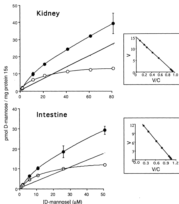
Fig. 4. Initial rate (15 s) of D-mannose uptake vs. increasing concentrations of external D-mannose. The composition of the intra- and extravesicular buffers was as described in Section 2. The values for the nonsaturable component (—) were determined by fitting the total transport data (●) to a transport model describing a single saturable system plus a nonsaturable component. The theoretically derived nonsaturable component was subtracted from total transport to calculate the saturable component (○). (Inserts) Eadie-Hofstee plots of the difference data. Mean values \pm S.E.M., n=4 .
