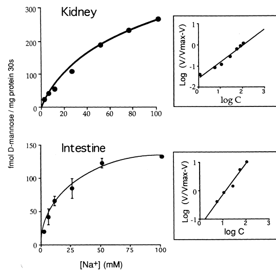
Fig. 5. Stoichiometry of \text{Na}^+ /D-mannose cotransport. 0.1 \mu\text{M} D-[ ^3\text{H} ]mannose uptake was measured for 30 s as a function of external \text{Na}^+ concentration. The BBMVs were loaded with a buffer containing, in mM: 200 mannitol, 50 KG and 50 HEPES-Tris (pH 7.5). The uptake buffer contained (in mM): 50 KG, 0.045 valinomycin, 50 HEPES-Tris (pH 7.5), 10^{-4} D-[ ^3\text{H} ]mannose, and 0–100 NaG with mannitol replacing NaG isosmotically. The \text{Na}^+ -dependent D-mannose uptake vs. extravesicular \text{Na}^+ concentration is shown. Mean values \pm S.E.M., n = 4 . (Inserts) Hill (log-log) plots of the data.
